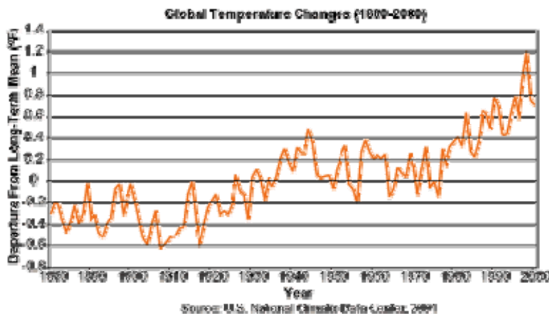
Figure 1. Global Average Temperature (EPA 2002)
